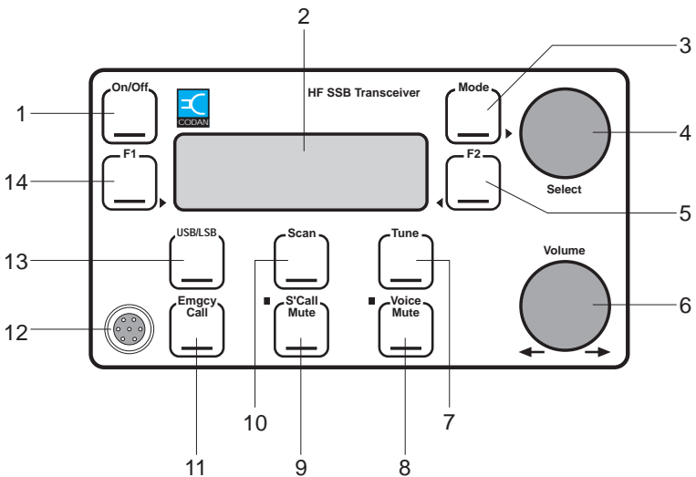
Figure 2.2 Control panel of the control head
