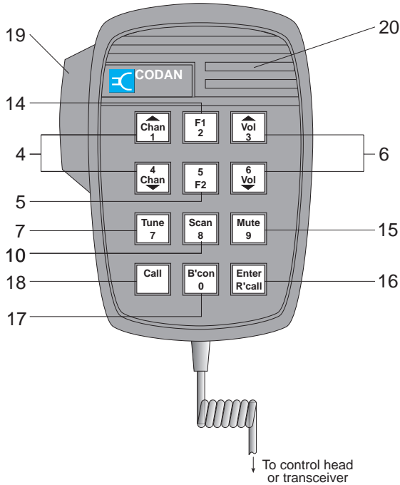
Figure 2.3 The microphone
