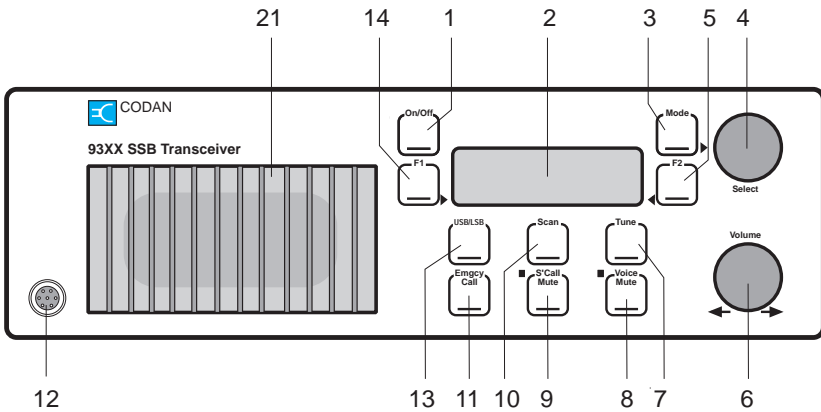
Figure 2.1 Front panel of the transceiver
