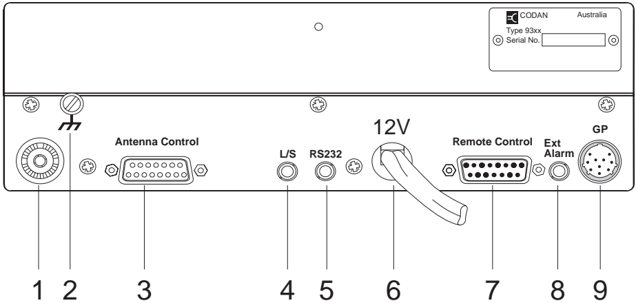
Figure 2.5 Rear panel of the transceiver
